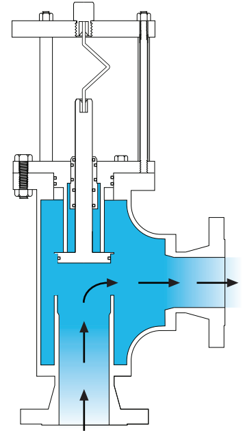
(Buckled Pin) Pressure Below Set Point
