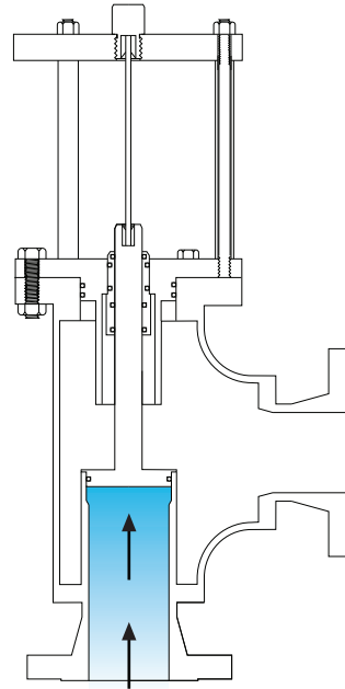
(Straight Pin) Pressure At Set Point
